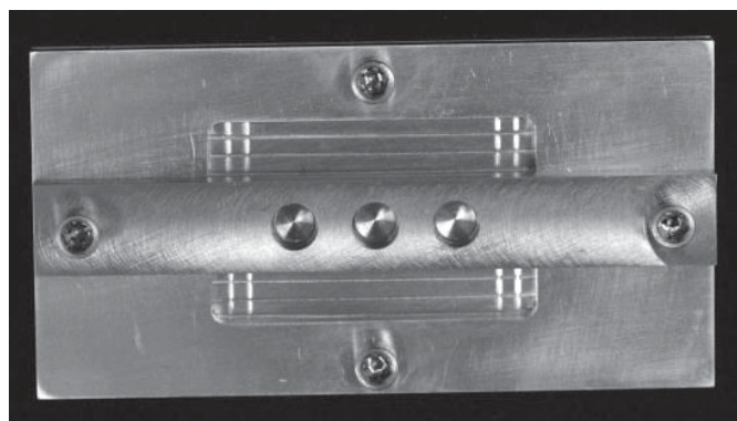
Fig. 1 – Matrix: 1- base with in line cylinders (3.75mm diameter x 4 mm height). 2: component with central opening level with the height of the cylinders. 3: rectangular bar with 3 holes coinciding with the location of the cylinders. Lateral screws to keep the three components stable.
