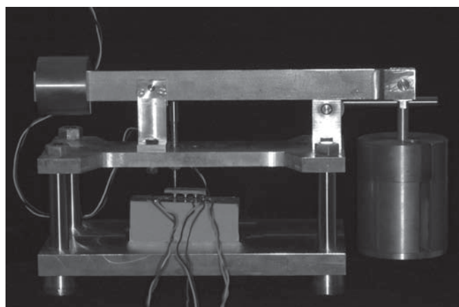
Fig. 3 - Experimental model in the loading apparatus with load applied at point A.
