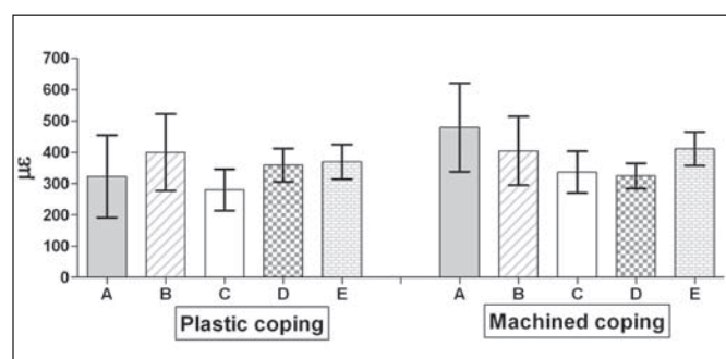
Fig. 5 - Mean values and standard deviations of the microstrain ( \mu\epsilon ) for plastic and machined copings in each load point.
