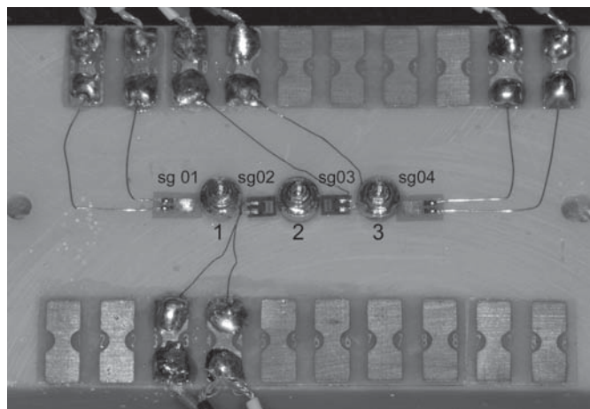
Fig. 2 - Strain gauges around the microunit abutments.
